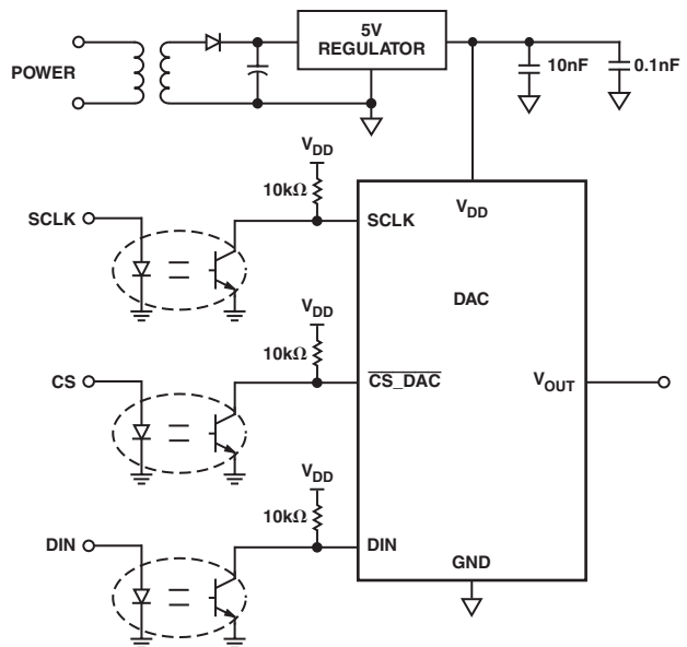
Figure 37. DAC in an Optocoupler Interface
