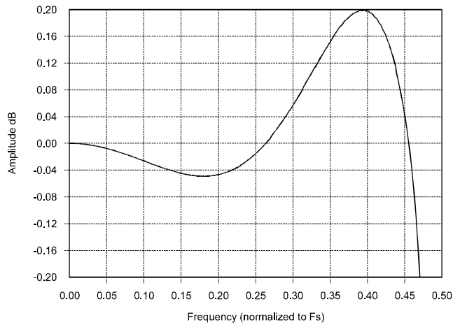
Figure 22. Passband Ripple
