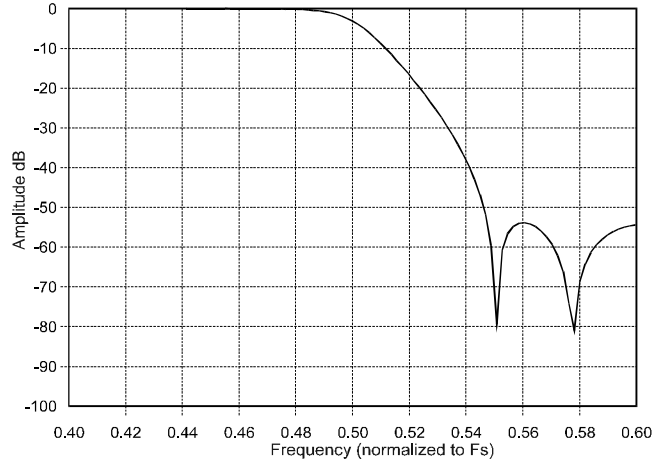
Figure 16. Transition Band
