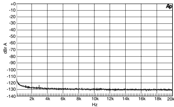
(16k FFT with no input signal) Figure 25. Idle Channel Noise FFT (BRM)
