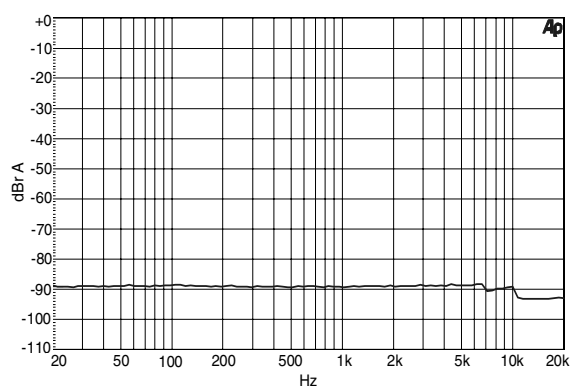
(THD+N plots measured using a 1kHz 24-bit dithered input signal) Figure 28. THD+N vs. Frequency (BRM)
