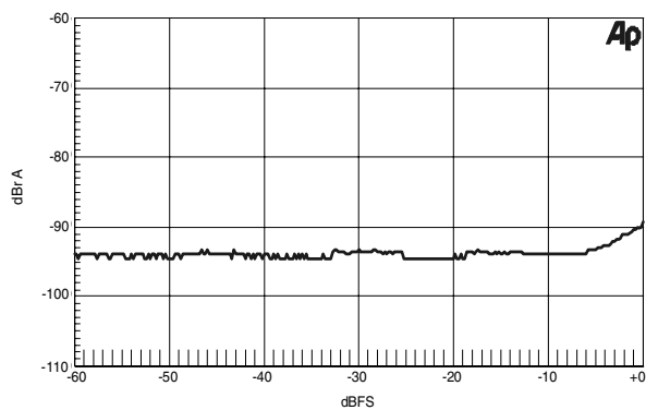
(THD+N plots measured using a 1kHz 24-bit dithered input signal) Figure 27. THD+N vs. Amplitude (BRM)
