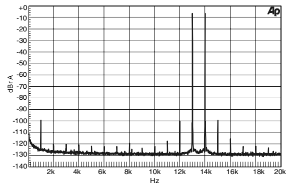
(16k FFT of intermodulation distortion using 13 kHz and 14 kHz input signals) Figure 26. Twin Tone IMD FFT (BRM)
