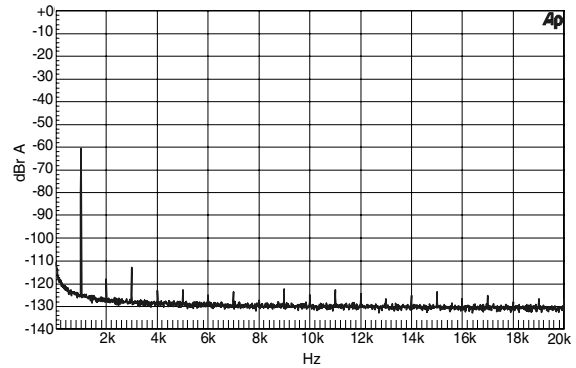
(16k FFT of a 1 kHz input signal) Figure 24. -60 dBFS FFT (BRM)
