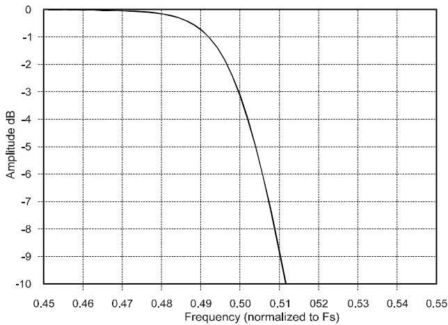
Figure 17. Transition Band
