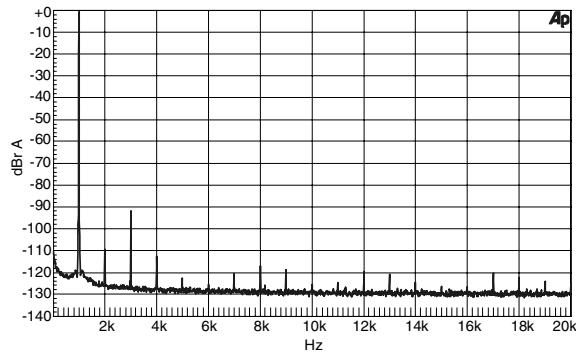
(16k FFT of a 1 kHz input signal) Figure 23. 0 dBFS FFT (BRM)
