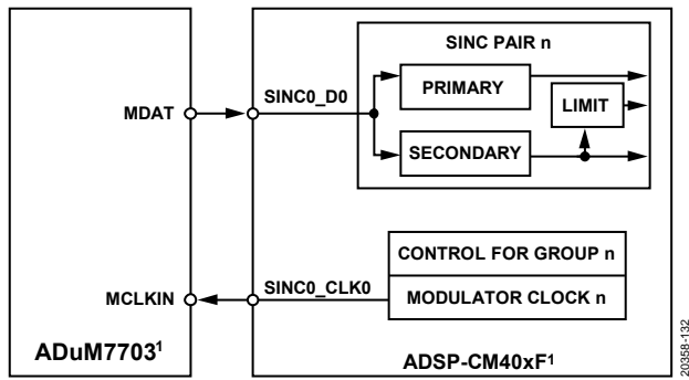
Figure 32. Interfacing the ADuM7703 to the ADSP-CM4xx
