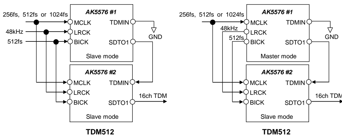
Figure 29. Cascade Connection
