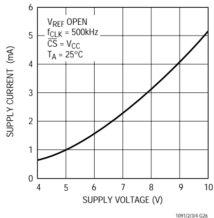
LTC1092/LTC1093/LTC1094 Supply Current vs Supply Voltage
