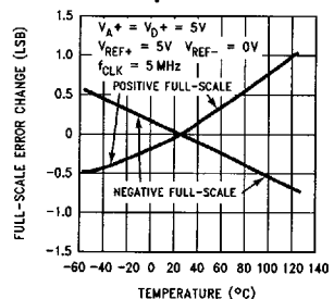
Full-Scale Error Change vs Temperature
