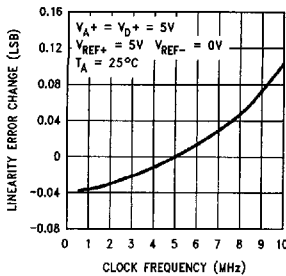
Linearity Error Change vs Clock Frequency
