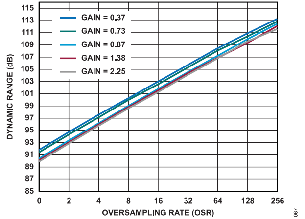
Figure 68. Dynamic Range vs. Oversampling Rate
