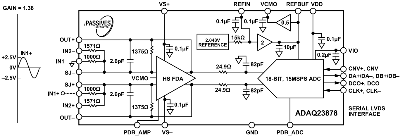
Figure 80. ADAQ23878 Single-Ended Input Configuration with Gain = 1.38
