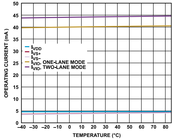
Figure 58. Operating Current vs. Temperature ( I_{VDD} = VDD Current, I_{VS+} = VS+ Current, I_{VS-} = VS- Current, I_{VIO} = VIO Current)
