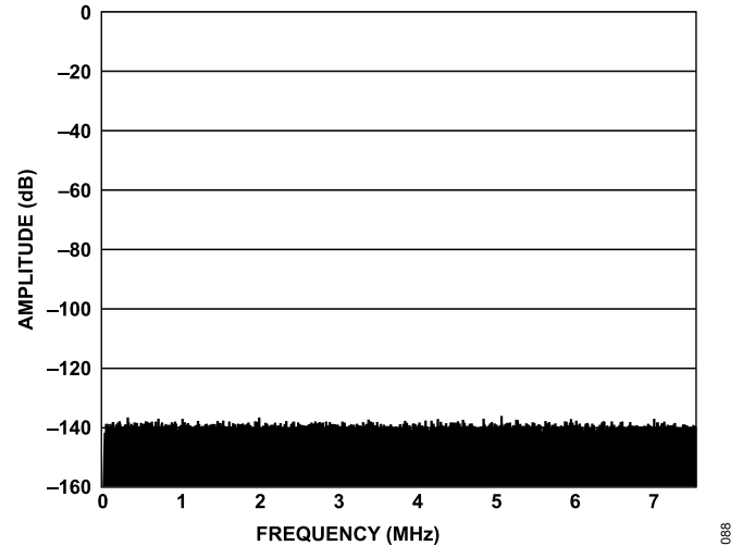
Figure 89. FFT with Shorted Inputs
