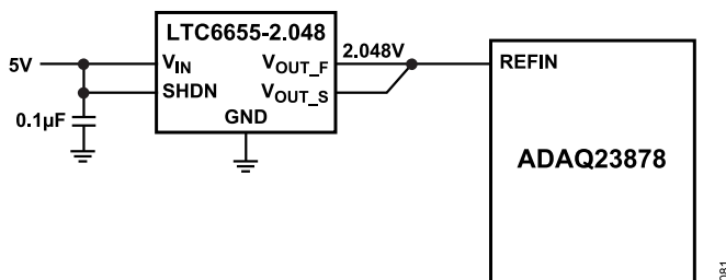
Figure 82. Using the LTC6655 as an External Reference
