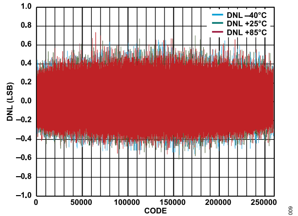
Figure 9. DNL vs. Code for Various Temperatures
