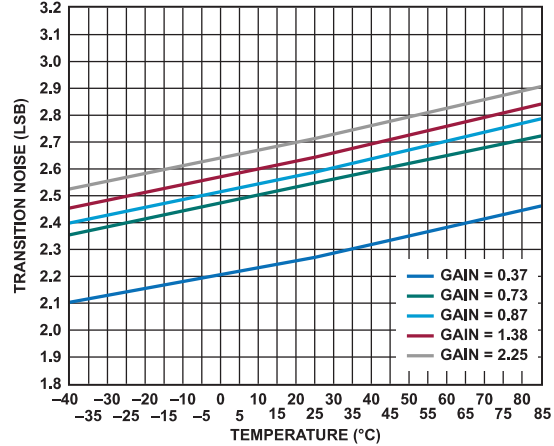
Figure 57. Transition Noise vs. Temperature, Gain
