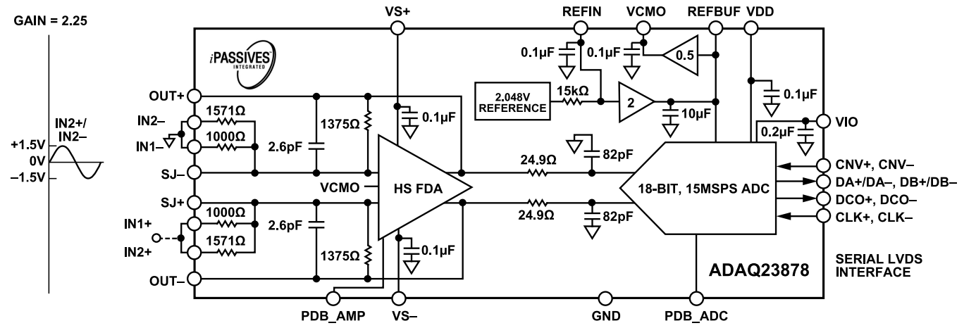
Figure 81. ADAQ23878 Single-Ended Input Configuration with Gain = 2.25
