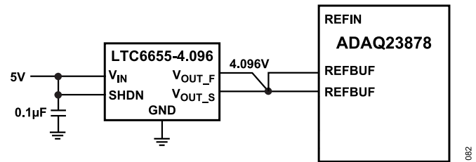
Figure 83. Overdriving REFBUF Using the LTC6655
