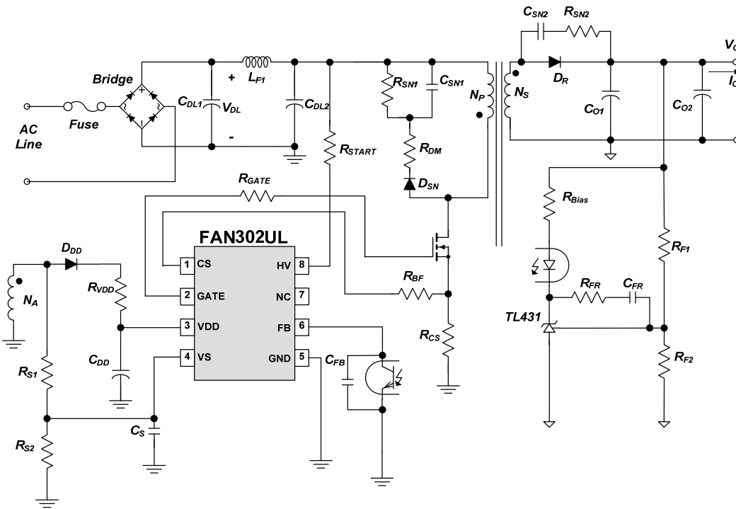
Figure 2. Typical Application
