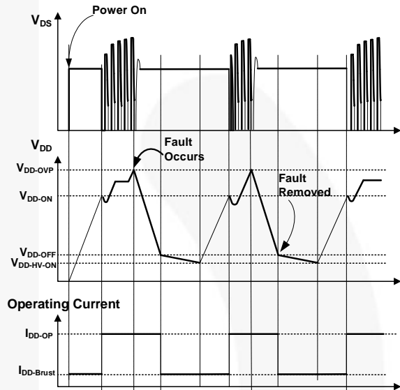
Figure 44. Auto-Restart Mode Operation
