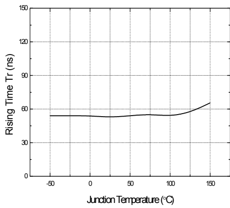
Figure 9. Output Rising Time
