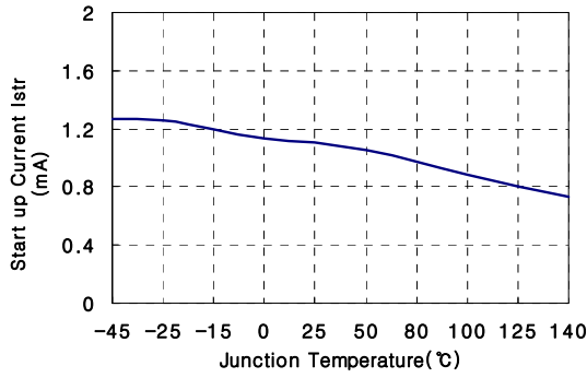
Figure 12. Startup Current
