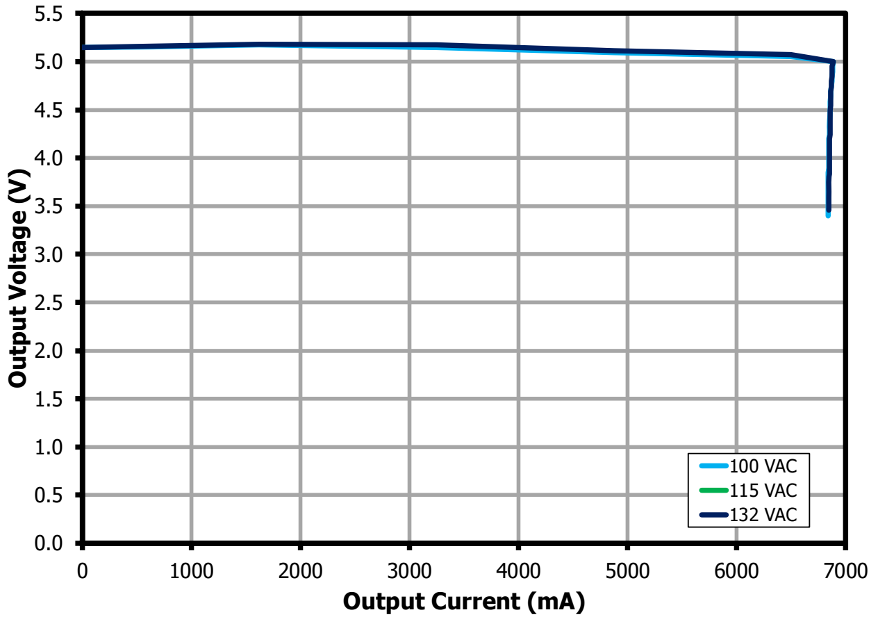
Figure 25 – VI Curve at V_{OUT} = 5\text{ V} .
