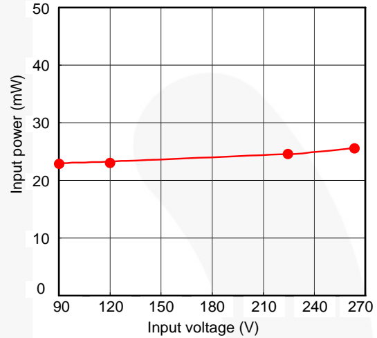
Figure 31. Standby Power
