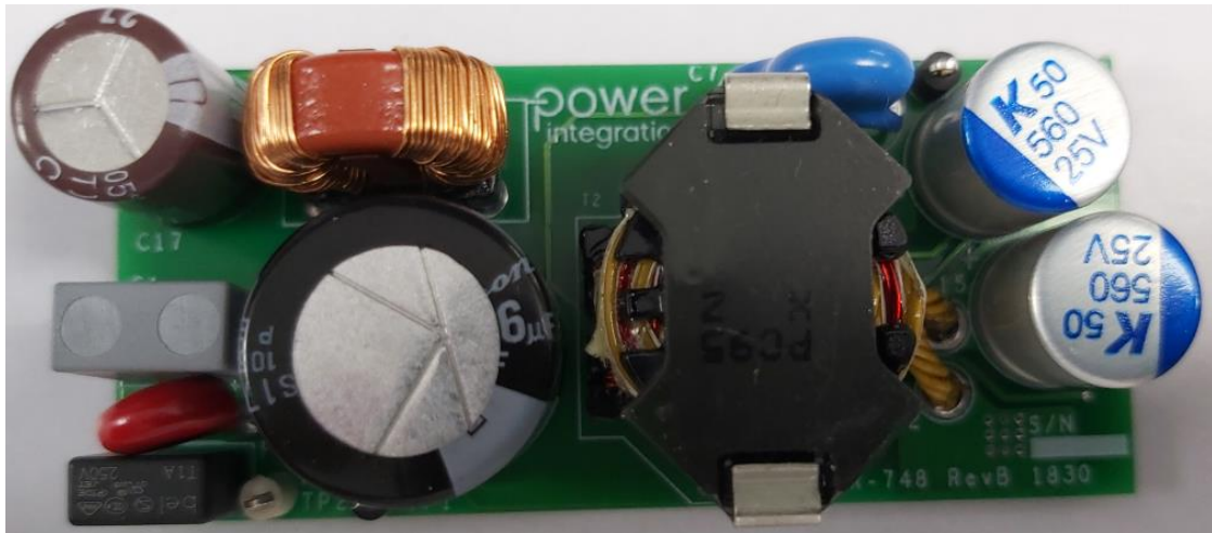
Figure 1 – Populated Circuit Board, Top View.
