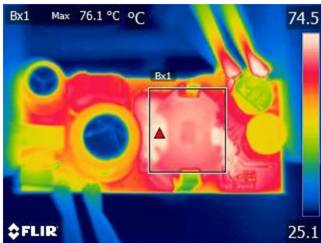
Figure 22 – Ambient = 25.1 °C. Transformer, T2 = 76.1 °C.
