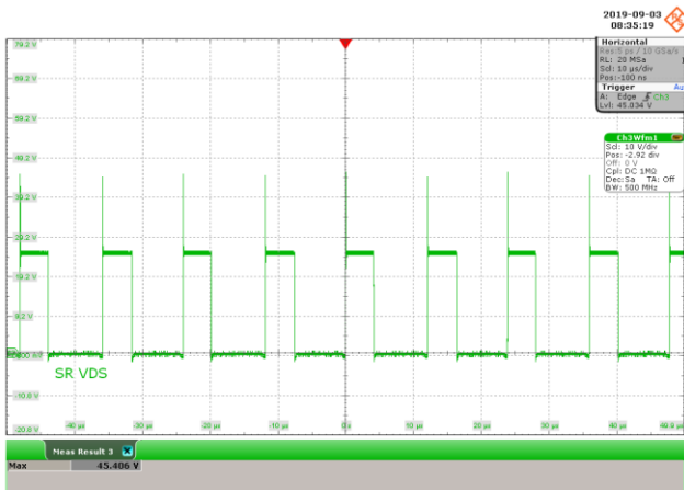
Figure 65 – SR1 FET Voltage Waveform. 100 VAC, 9 V, 5.0 A Load, (45.406 V MAX ). V DRAIN , 10 V, 10 μs / div.
