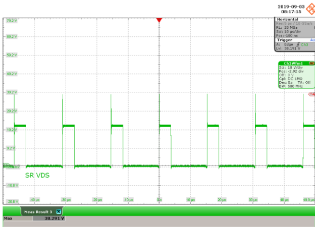
Figure 63 – SR FET Voltage Waveform. 100 VAC, 5 V, 6.5 A Load, (38.291 V MAX ). V DRAIN , 10 V, 10 μs / div.
