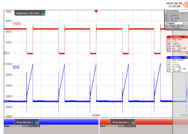
Figure 52 – Drain Voltage and Current Waveforms. 135 VAC, 5 V, 6.5 A Load, (271 V MAX ). Upper: V DRAIN , 100 V, 10 μs / div. Lower: I DRAIN , 500 mA / div.
