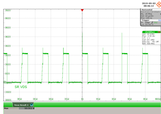
Figure 66 – SR1 FET Voltage Waveform. 135 VAC, 9 V, 5.0 A Load, (53.311 V MAX ). V DRAIN , 10 V, 10 μs / div.
