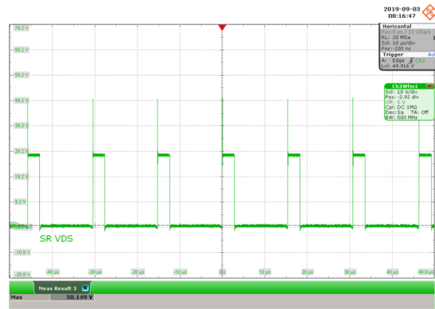
Figure 64 – SR FET Voltage Waveform. 135 VAC, 5 V, 6.5 A Load, (50.149 V MAX ). V DRAIN , 10 V, 10 μs / div.
