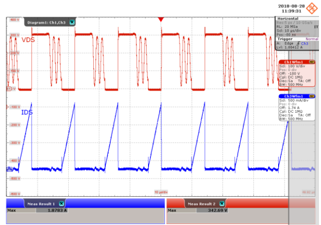
Figure 56 – Drain Voltage and Current Waveforms. 135 VAC, 15.0 V, 3.0 A Load, (343 V MAX ). Upper: V DRAIN , 100 V, 10 μs / div. Lower: I DRAIN , 500 mA / div.
