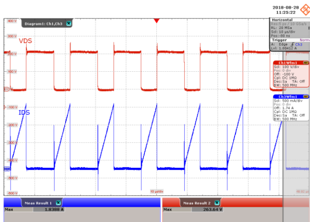
Figure 53 – Drain Voltage and Current Waveforms. 100 VAC, 9.0 V, 5.0 A Load, (264 V MAX ). Upper: V DRAIN , 100 V, 10 μs / div. Lower: I DRAIN , 500 mA / div.
