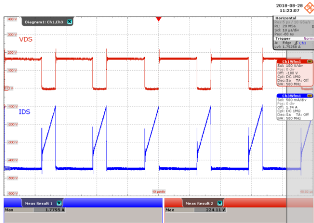
Figure 51 – Drain Voltage and Current Waveforms. 100 VAC, 5 V, 6.5 A Load, (224 V MAX ). Upper: V DRAIN , 100 V, 10 μs / div. Lower: I DRAIN , 500 mA / div.
