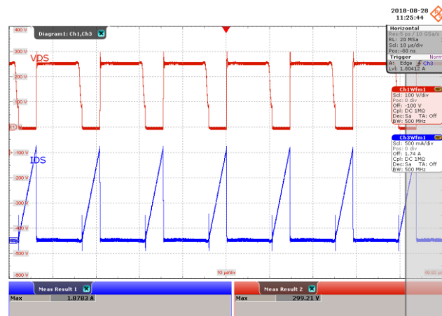
Figure 54 – Drain Voltage and Current Waveforms. 135 VAC, 9.0 V, 5.0 A Load, (299 V MAX ). Upper: V DRAIN , 100 V, 10 μs / div. Lower: I DRAIN , 500 mA / div.
