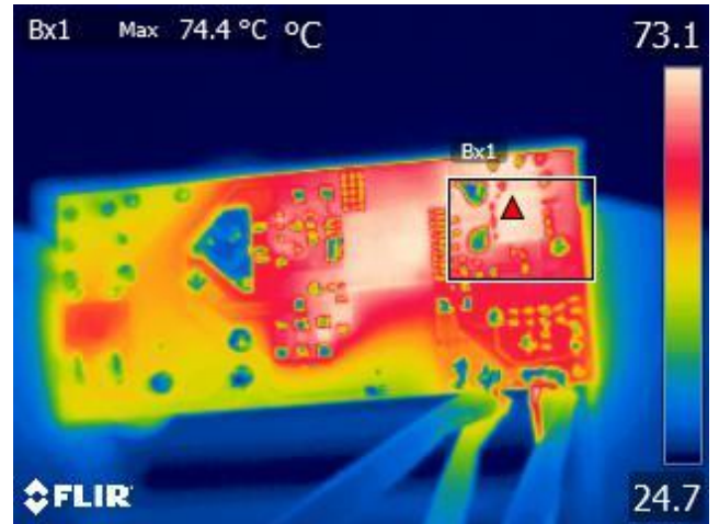
Figure 25 – Ambient = 24.7 °C. SR FET, Q3 = 74.4 °C.
