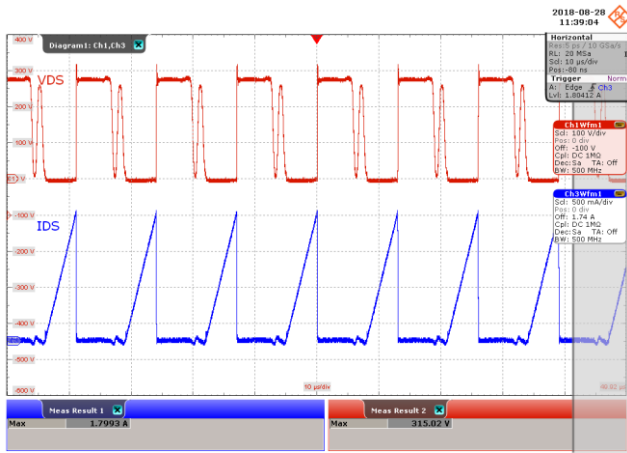
Figure 55 – Drain Voltage and Current Waveforms. 100 VAC, 15.0 V, 3.0 A Load, (315 V MAX ). Upper: V DRAIN , 100 V, 10 μs / div. Lower: I DRAIN , 500 mA / div.
