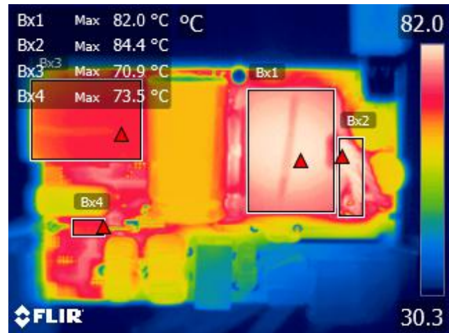
Figure 55 – Top Thermal Image, T_{AMB} = 28.3\text{ }^{\circ}\text{C} . Bx1: Transformer Core = 82.0 °C. Bx2: Transformer Wire = 84.4 °C. Bx3: PFC Inductor Core = 70.9 °C. Bx4: Boost Pre-charge Diode = 73.5 °C.
