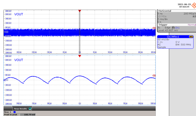
Figure 115 – Output Voltage Ripple. 265 VAC, 5.0 V, 5 A Load. V_{OUT(AC)} = 100 mV Peak-to-Peak. CH1: V_{OUT(AC)} , 50 mV / div. Time: 5 ms / div. (25 \mu s / div. Zoom).
