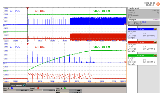
Figure 77 – SR FET Drain Voltage and Current. 265 VAC, 5.0 V, 5 A (CR Mode, 930 mΩ at the End of 100 mΩ Cable). V_{DS\_SRFET} = 113.8\text{ V} Maximum. CH1: V_{DS\_SRFET} , 40 V / div. CH2: I_{DS\_SRFET} , 10 A / div. CH4: V_{BUS\_IN} , 1 V / div. Time: 100 ms / div. (200 μs / div. Zoom).
