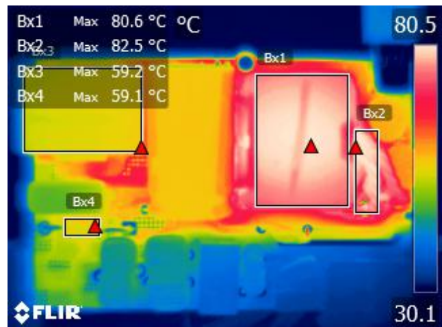
Figure 57 – Top Thermal Image, T_{AMB} = 28.8\text{ }^{\circ}\text{C} . Bx1: Transformer Core = 80.6 °C. Bx2: Transformer Wire = 82.5 °C. Bx3: PFC Inductor Core = 59.2 °C. Bx4: Boost Pre-charge Diode = 59.1 °C.
