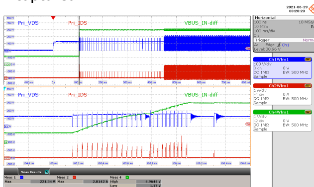
Figure 74 – Primary Drain Voltage and Current. 90 VAC, 5.0 V, 5 A (CR Mode, 880 mΩ at the End of 100 mΩ Cable). V_{DS\_PRI} = 221\text{ V} Maximum. CH1: V_{DS\_PRI} , 100 V / div. CH2: I_{DS\_PRI} , 1 A / div. CH4: V_{BUS\_IN} , 1 V / div. Time: 100 ms / div. (200 μs / div. Zoom).
