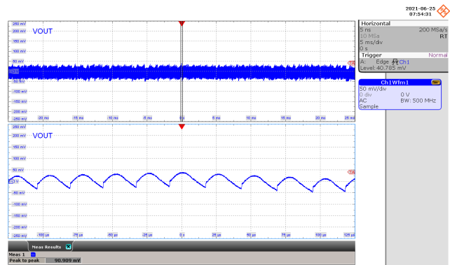
Figure 119 – Output Voltage Ripple. 265 VAC, 12.0 V, 5 A Load. V_{OUT(AC)} = 90 mV Peak-to-Peak. CH1: V_{OUT(AC)} , 50 mV / div. Time: 5 ms / div. (25 \mu s / div. Zoom).
