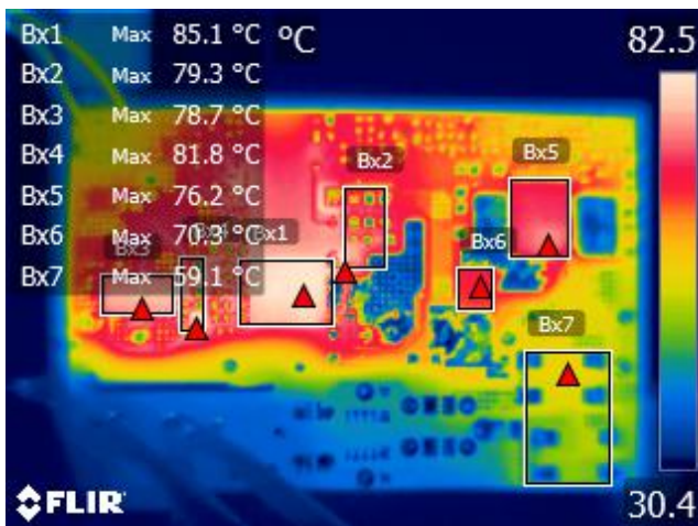
Figure 56 – Bottom Thermal Image, T_{AMB} = 28.9\text{ }^{\circ}\text{C} . Bx1: InnoSwitch3-PD = 85.1 °C. Bx2: Primary Clamp = 79.3 °C. Bx3: SR FET = 78.7 °C. Bx4: SR FET Snubber = 81.8 °C. Bx5: HiperPFS-4 = 76.2 °C. Bx6: PFC Boost Diode = 70.3 °C. Bx7: Bridge Rectifier = 59.1 °C.
