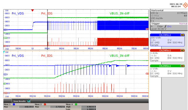
Figure 75 – Primary Drain Voltage and Current. 265 VAC, 5.0 V, 5 A (CR Mode, 880 mΩ at the End of 100 mΩ Cable). V_{DS\_PRI} = 450\text{ V} Maximum. CH1: V_{DS\_PRI} , 200 V / div. CH2: I_{DS\_PRI} , 1 A / div. CH4: V_{BUS\_IN} , 1 V / div. Time: 100 ms / div. (200 μs / div. Zoom).
