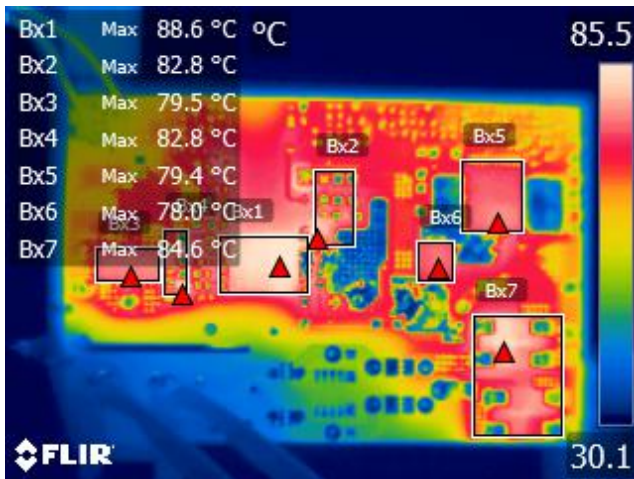
Figure 54 – Bottom Thermal Image, T_{AMB} = 28.0\text{ }^{\circ}\text{C} . Bx1: InnoSwitch3-PD = 88.6 °C. Bx2: Primary Clamp = 82.8 °C. Bx3: SR FET = 79.5 °C. Bx4: SR FET Snubber = 82.8 °C. Bx5: HiperPFS-4 = 79.4 °C. Bx6: PFC Boost Diode = 78.0 °C. Bx7: Bridge Rectifier = 84.6 °C.
