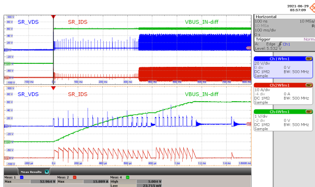
Figure 76 – SR FET Drain Voltage and Current. 90 VAC, 5.0 V, 5 A (CR Mode, 930 mΩ at the End of 100 mΩ Cable). V_{DS\_SRFET} = 52.9\text{ V} Maximum. CH1: V_{DS\_SRFET} , 20 V / div. CH2: I_{DS\_SRFET} , 10 A / div. CH4: V_{BUS\_IN} , 1 V / div. Time: 100 ms / div. (200 μs / div. Zoom).
